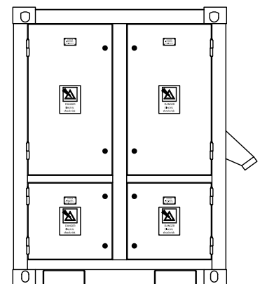
LEFT-SIDE VIEW
