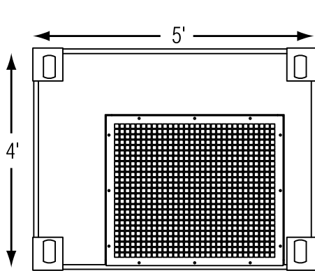
PLAN VIEW/FOOTPRINT
